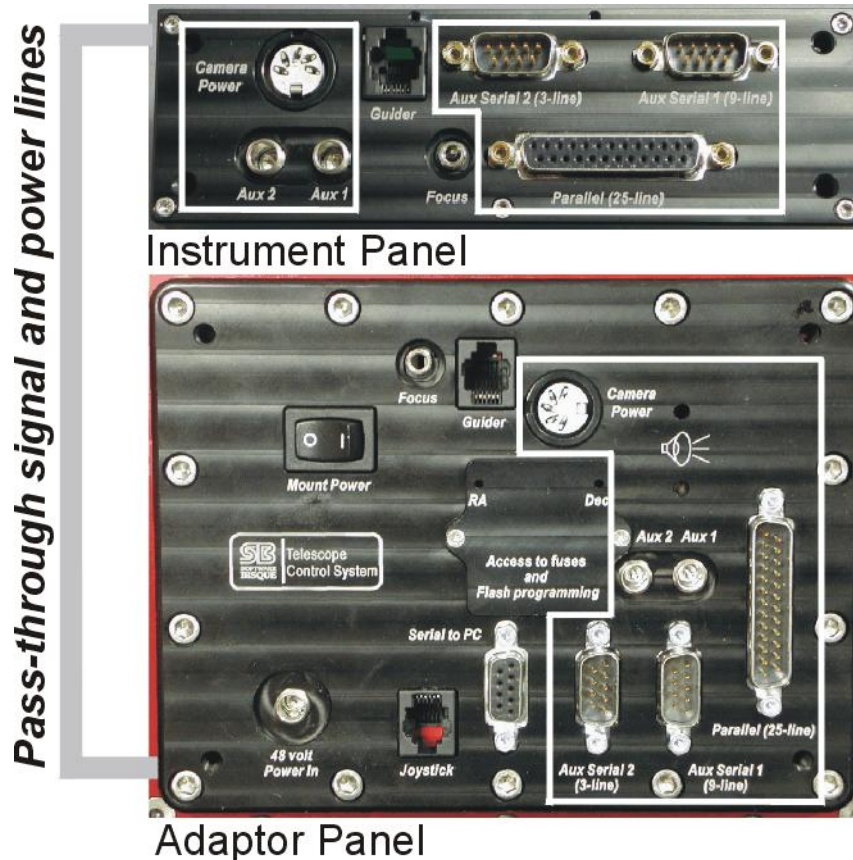
Figure 33: Relationship between Adapter Panel and Instrument Panel ports.
