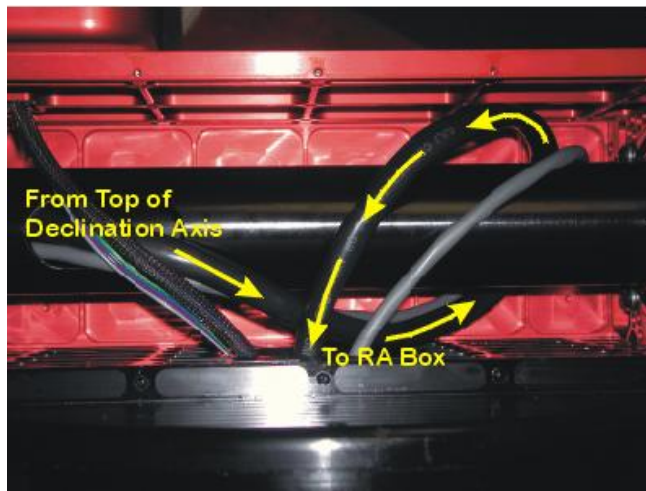
Figure 37: Make sure to loop the cable around the declination shaft.
