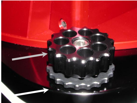
Figure 15: Micro-Leveler (white arrow) and Base Plate Attachment Knob (gray)
