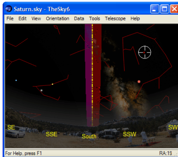
Figure 53: If you've successfully synchronized the Paramount ME, the shaded regions will be centered on the meridian.
