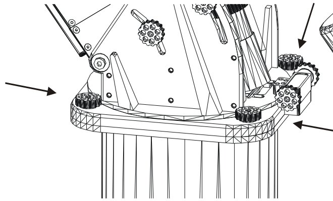
Figure 17: Location of Base Plate Attachment Knobs.
