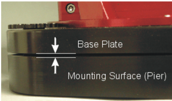
Figure 16: Adjusting Micro-Levelers.
