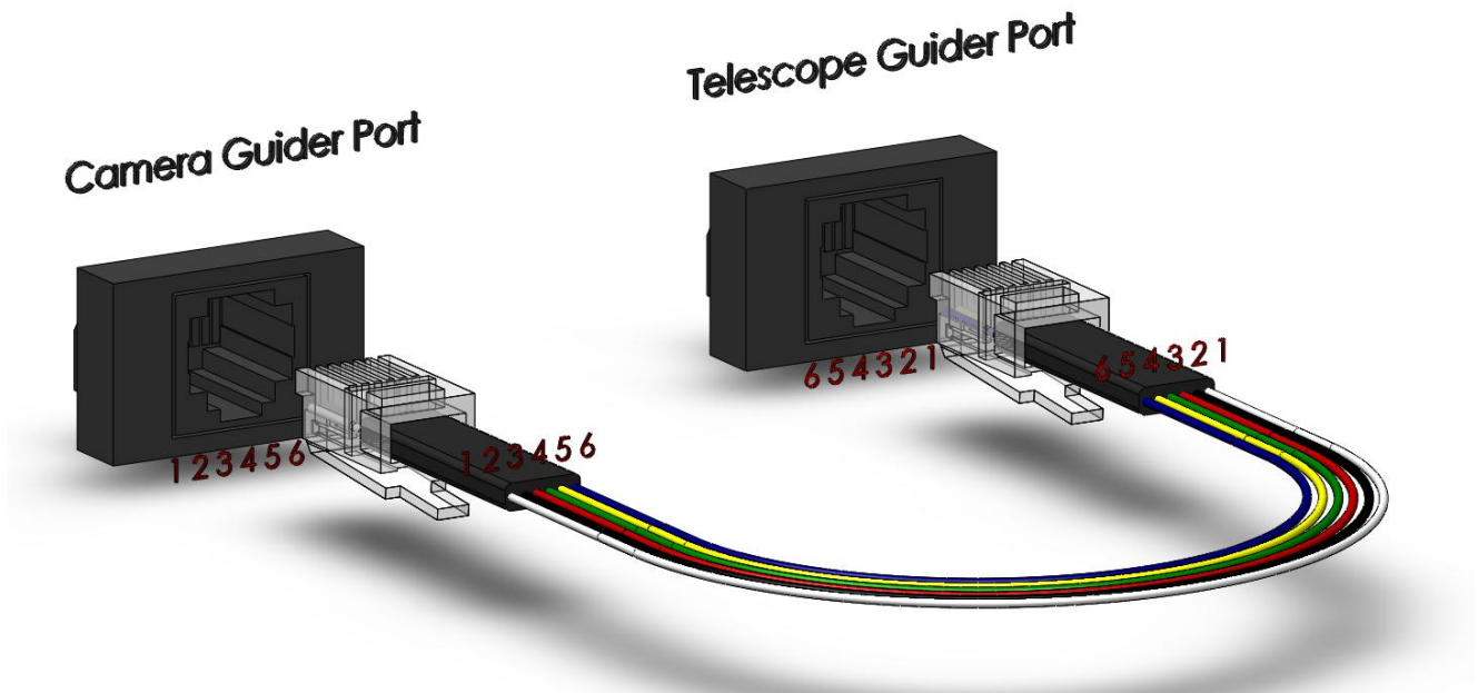
Figure 74: Diagram showing the pinouts for the guider cable and the camera and guider ports.
